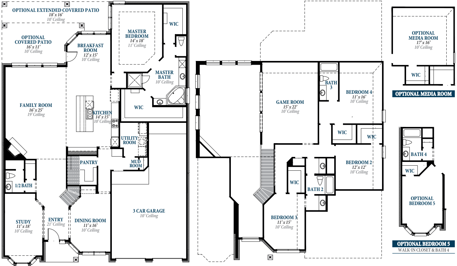
• FIRST FLOOR •
