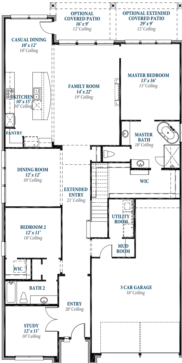
• FIRST FLOOR •
