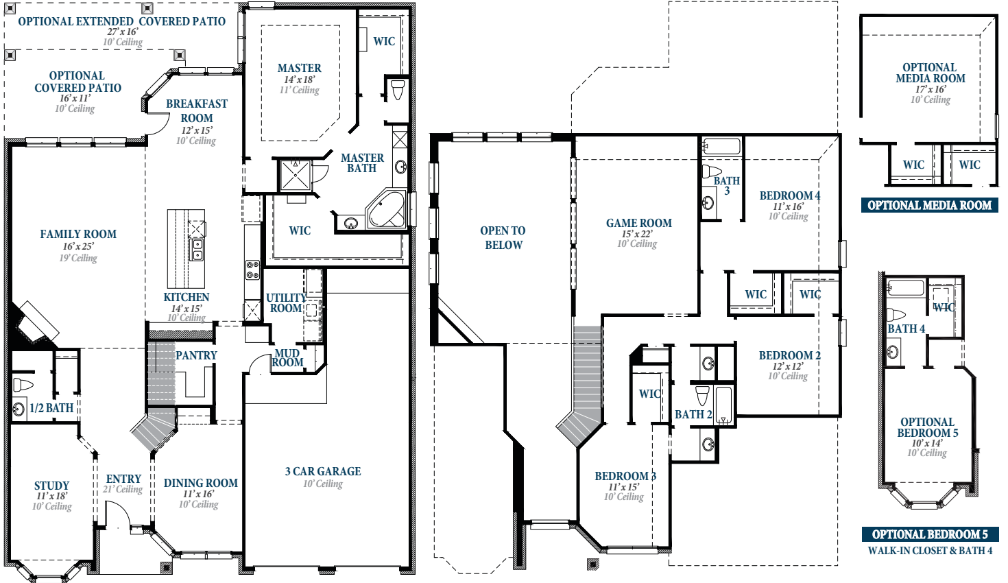
• FIRST FLOOR •
