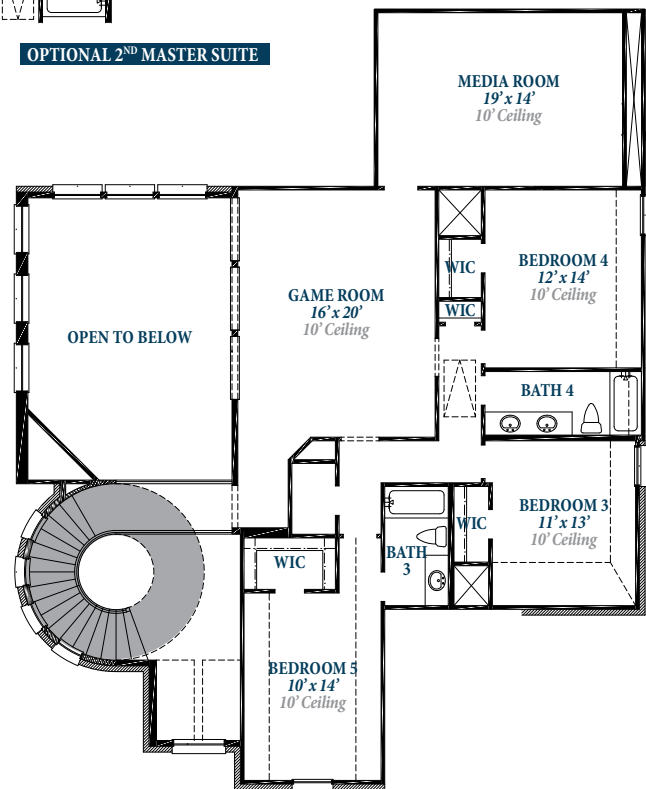
• SECOND FLOOR •
