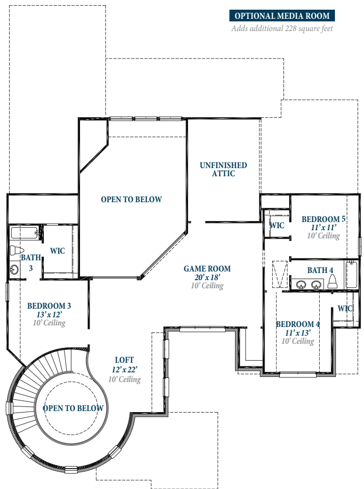
• SECOND FLOOR •
