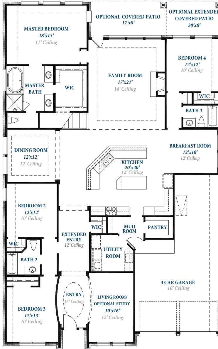
• FIRST FLOOR •
