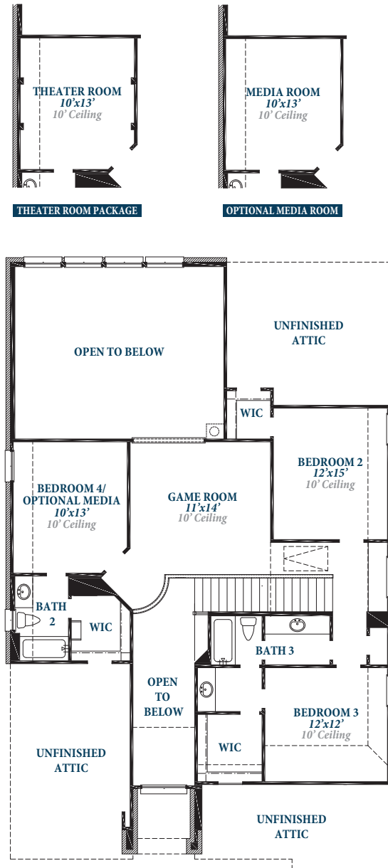
• SECOND FLOOR •
