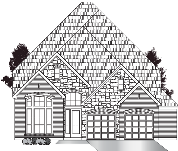
• ELEVATION B1 •
