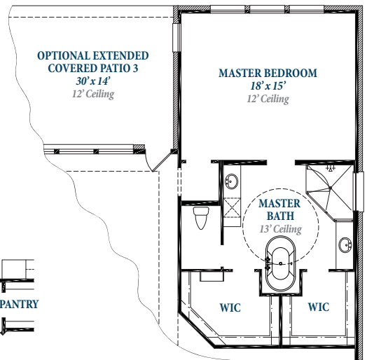
OPTIONAL MASTER SUITE 3 Requires Extended Covered Patio 3 Adds additional 139 square feet
